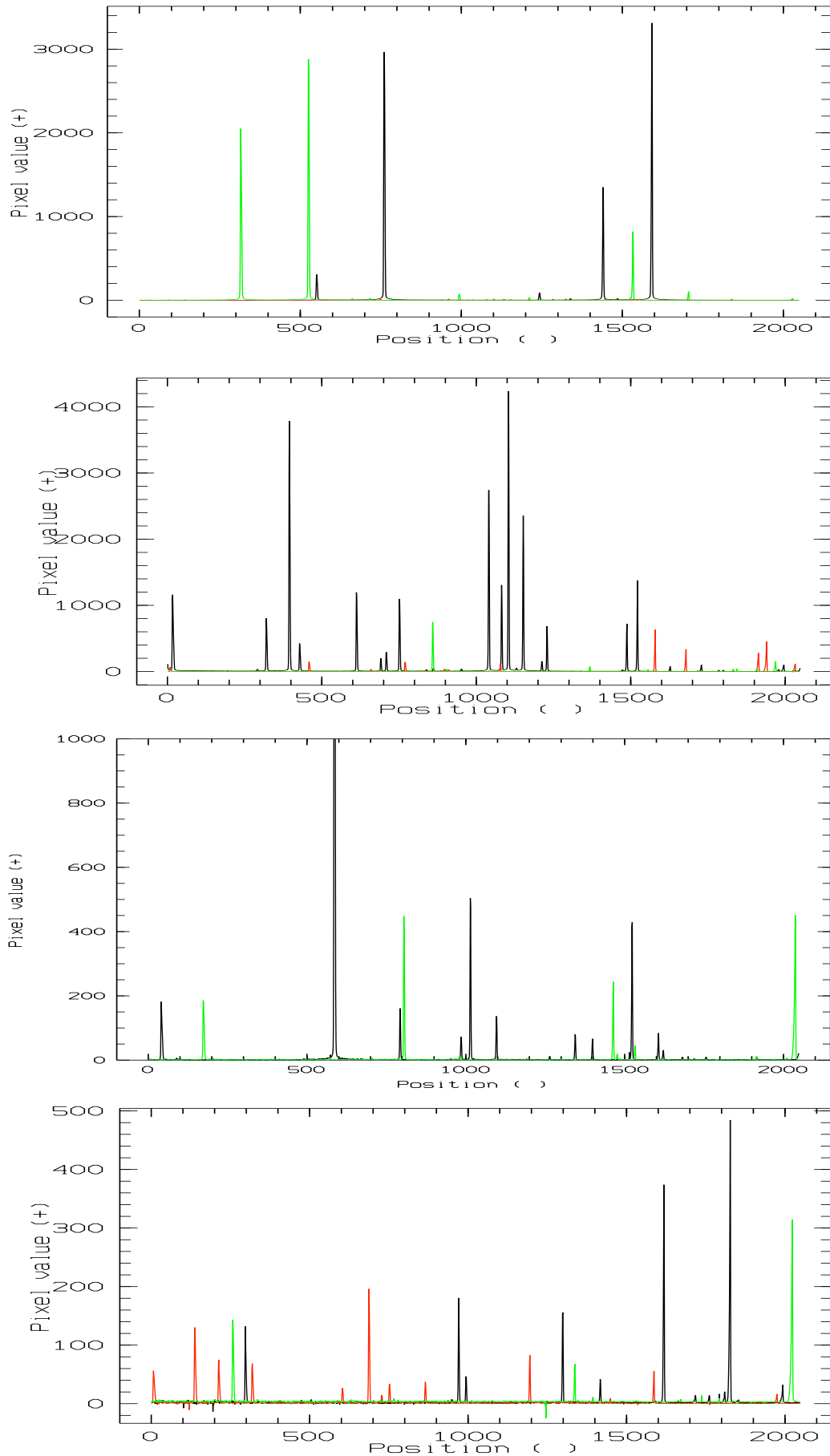
Figure 18: Calibration lines measured with the LS150 (0.25") slit for the 210_zJHK grating. Ar is represented in black, Xe green and Ne red (when available). From top to bottom: z Band, J band, H band & K band.
