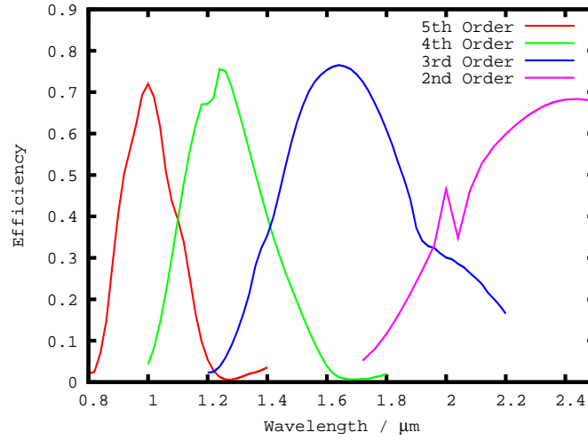
Figure 24: The efficiency of the 210_zJHK grating versus the wavelength, in Littrow configuration. The different orders (5th - 2nd) of the grating are color coded.
