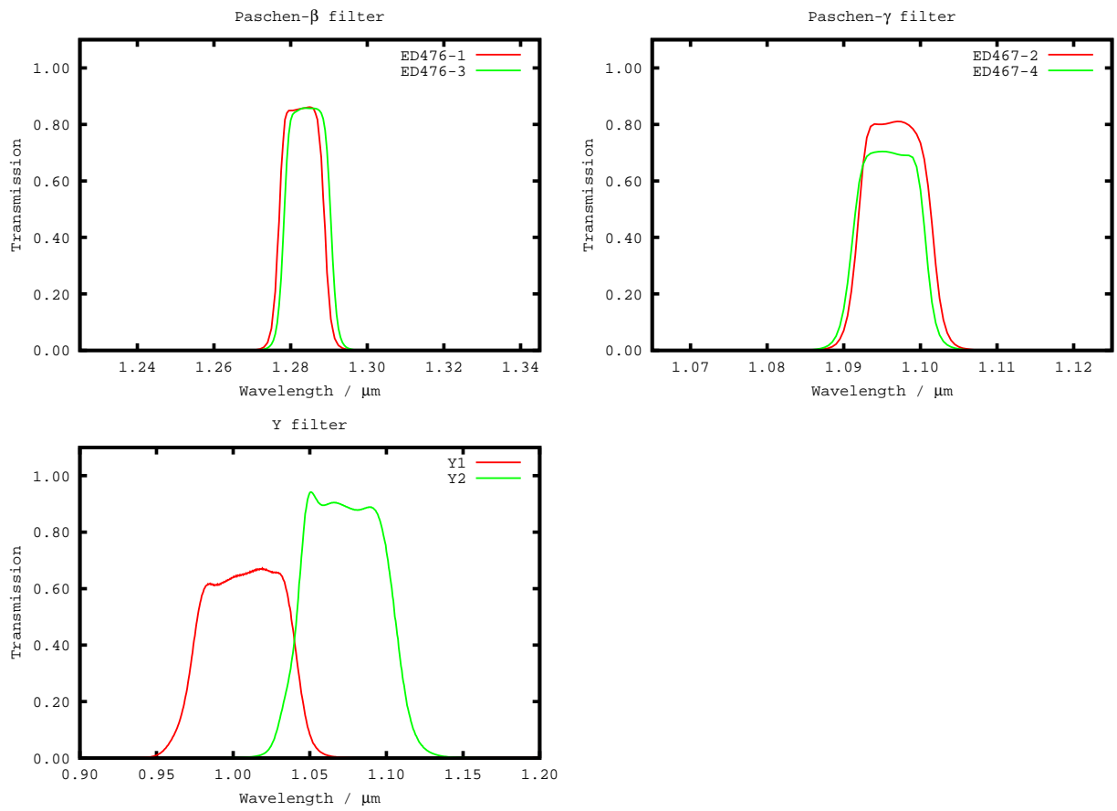
Figure 28: Narrow band filter curves (Part 2). If not otherwise specified, the red curves are the filters present in LUCIFER1. When specified, e.g. for Y1/Y2, then both filters are present in LUCIFER1.
