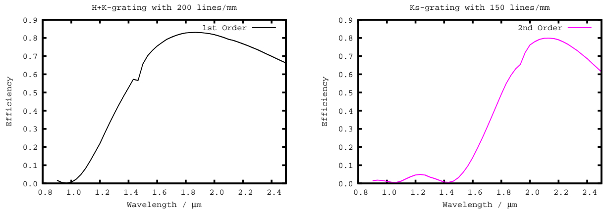
Figure 25: Grating efficiency versus wavelength, in Littrow configuration: 200_H+K grating left, 150_Ks right.
