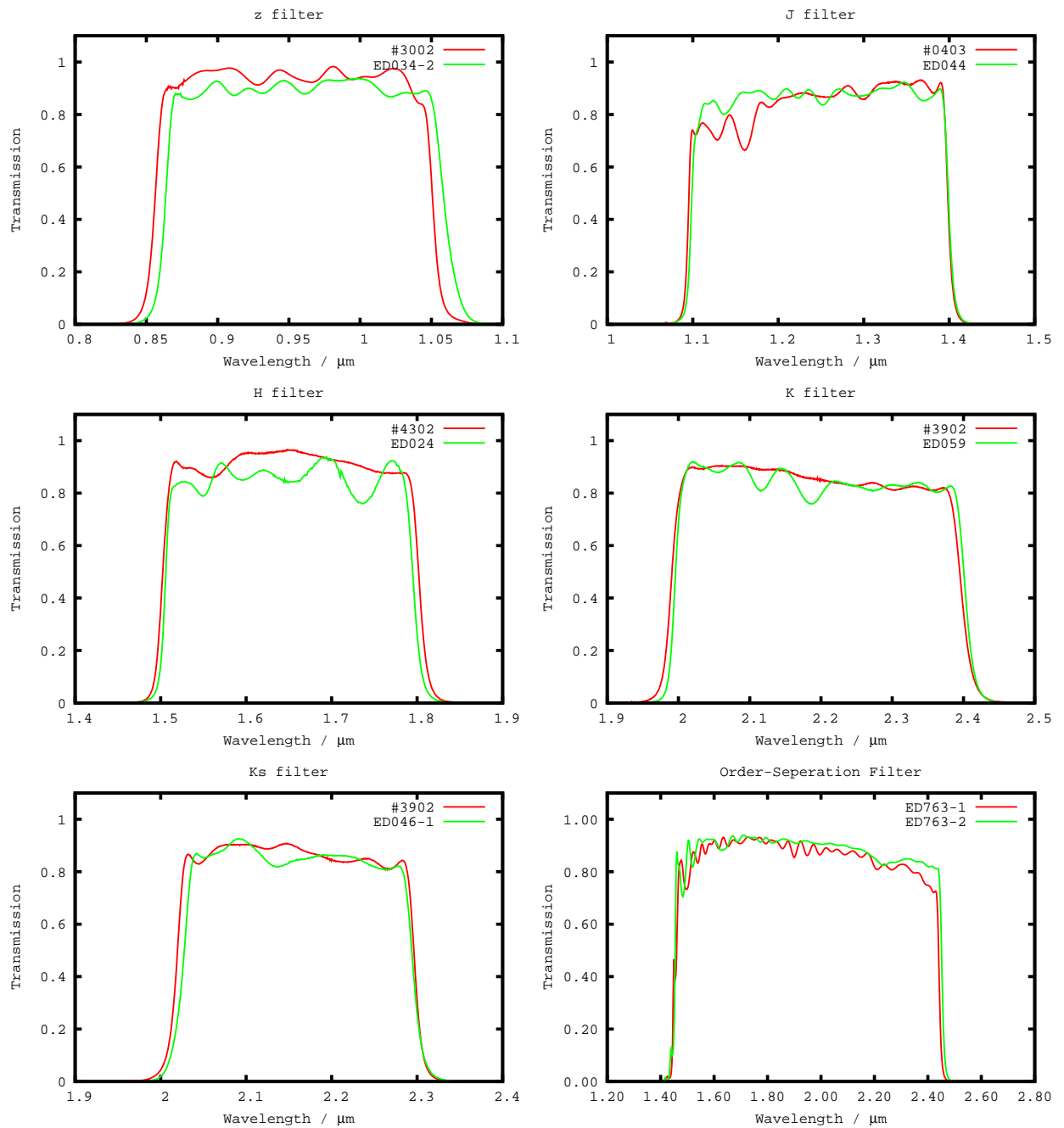
Figure 26: Filter curves for broad-band filters. (Red = filters installed in LUCIFER1)
