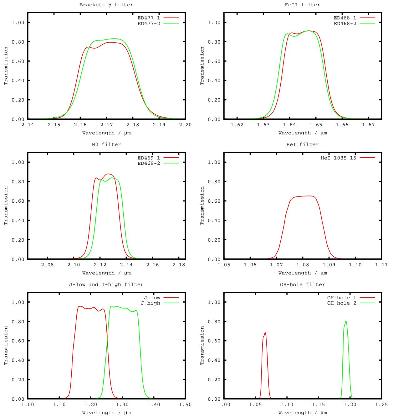
Figure 27: Narrow band filter curves (Part 1).
